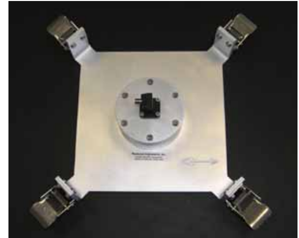
Waveguide-to-Coax SMA Adapter, Ceragon (23 GHz)
