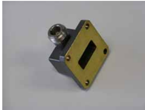
Waveguide-to-Coax Adapter WR-90 to 'N' (f) (8.20–12.40 GHz)
